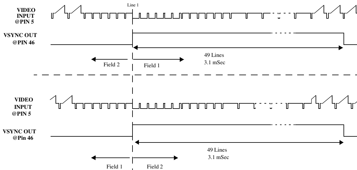
Figure 5 - VSync Output
