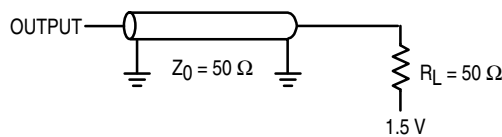
Figure 1. AC Test Load
