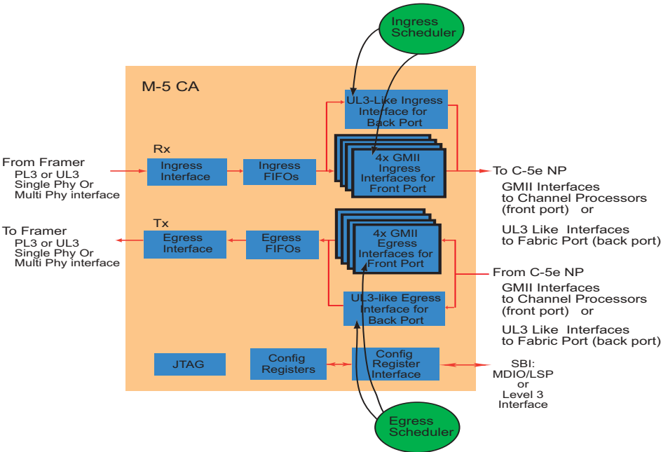
Figure 1 M-5 CA Functional Block Diagram
