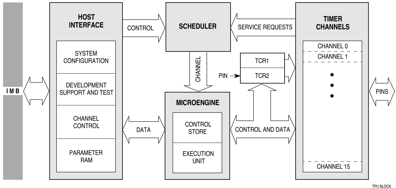
Figure 8 TPU Simplified Block Diagram
