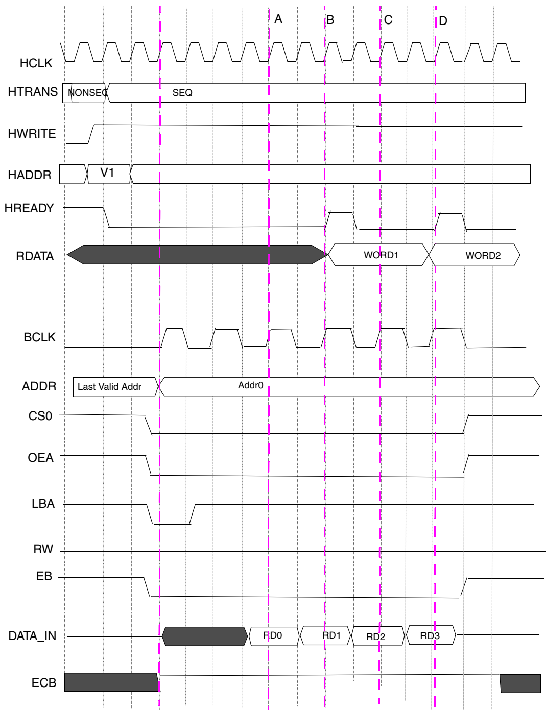
Figure 60. FCE=0,SYNC=1,BCD=1,WSC=4,BCS=0,CSA=0,OEA=0
