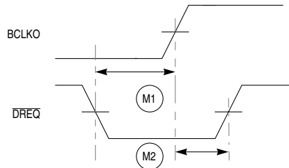
Figure 20-18. DMA Timing
