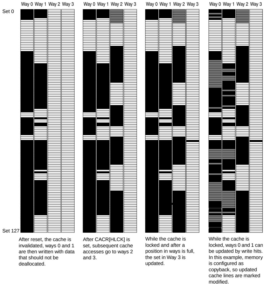
Figure 4-7. Cache Locking
