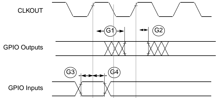
Figure 16. GPIO Timing
