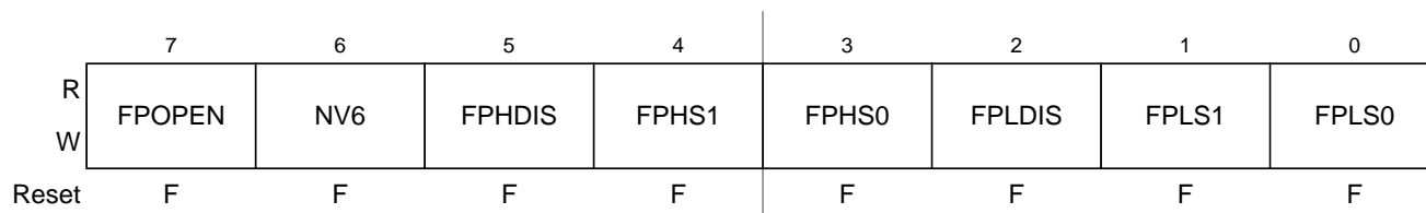
Figure 20-8. Flash Protection Register (FPROT)
