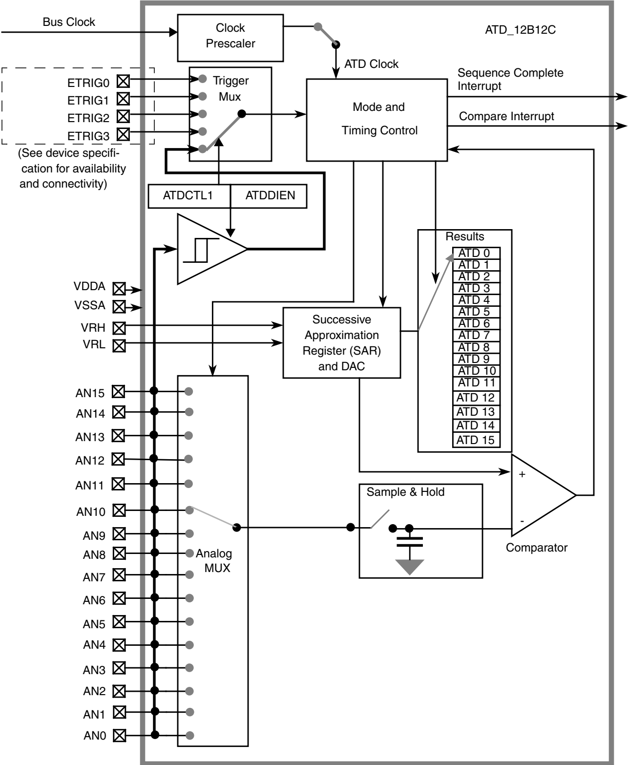
Figure 14-1. ADC12B16C Block Diagram
