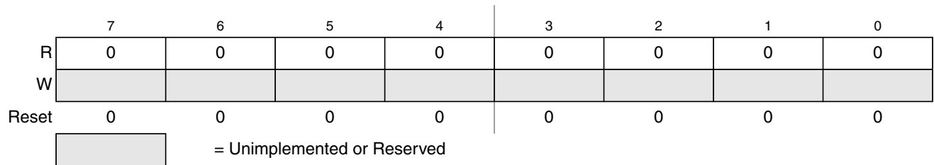
Figure 23-25. Flash Reserved7 Register (FRSV7)
