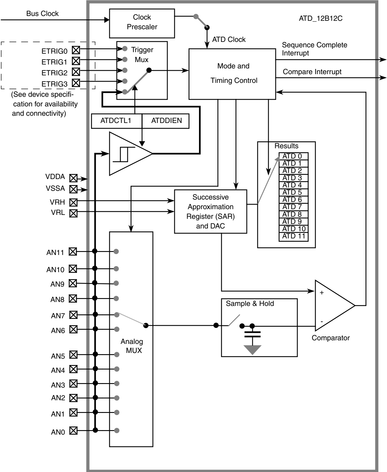
Figure 12-1. ADC10B12CV2 Block Diagram
