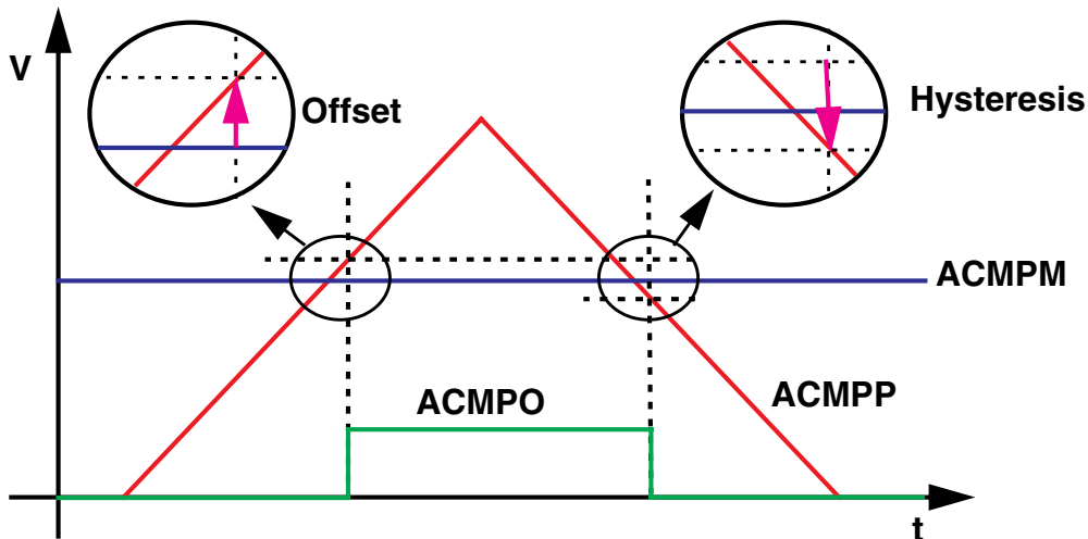
Figure A-2. Input Offset and Hysteresis
