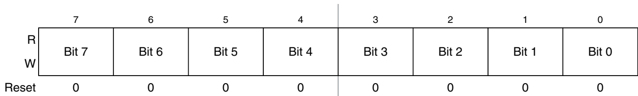
Figure 20-23. Timer Input Capture/Output Compare Register x Low (TCxL)
