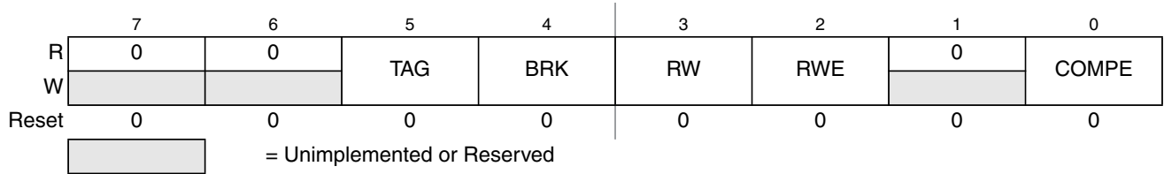
Figure 8-15. Debug Comparator Control Register DBGCTL (Comparator C)
