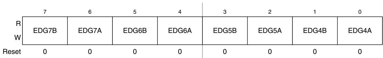
Figure 20-16. Timer Control Register 3 (TCTL3)
