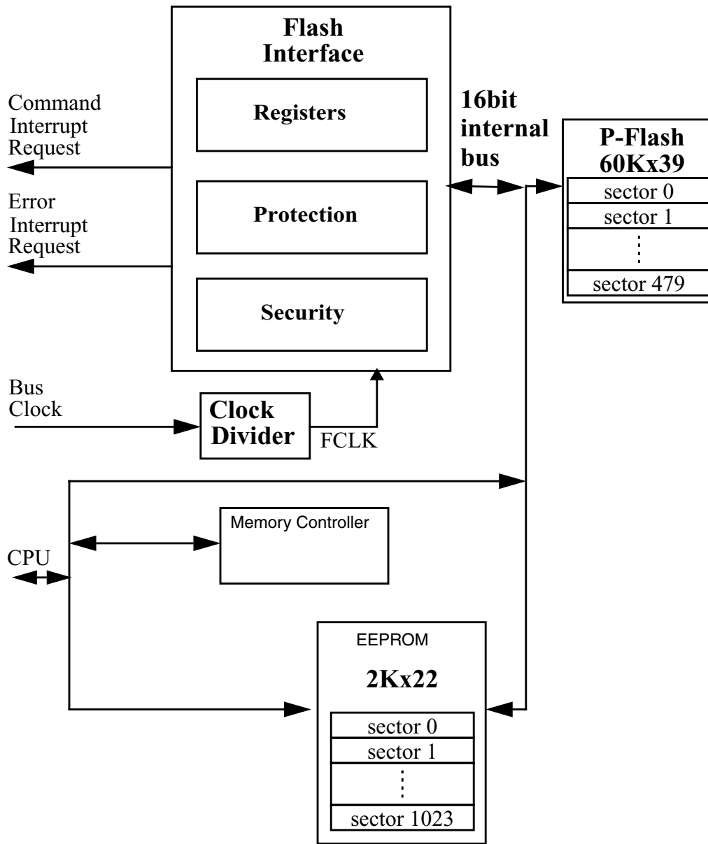
Figure 28-1. FTMRG240K2 Block Diagram
