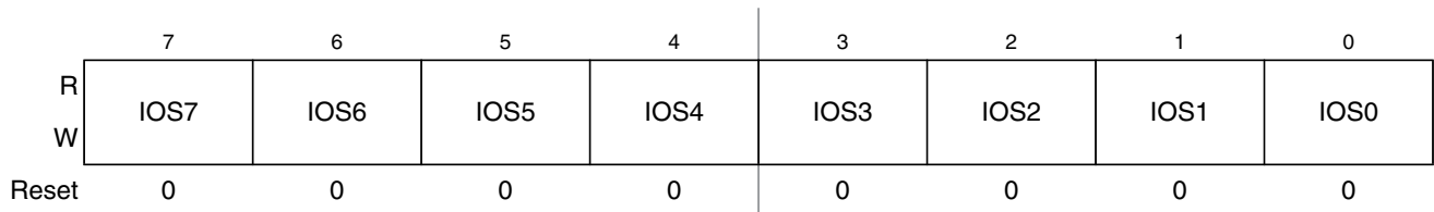
Figure 20-6. Timer Input Capture/Output Compare Select (TIOS)
