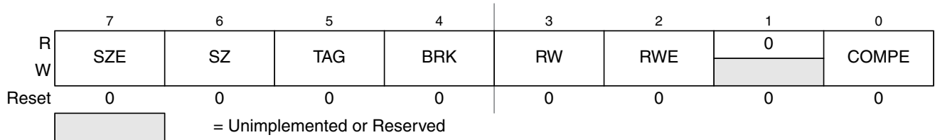
Figure 8-14. Debug Comparator Control Register DBGCTL (Comparator B)
