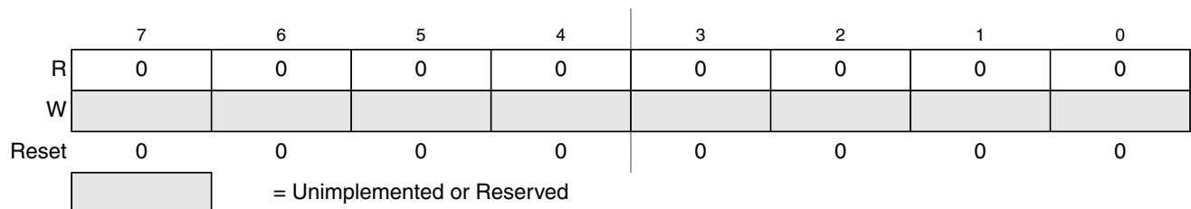
Figure 21-8. Flash Reserved0 Register (FRSV0)
