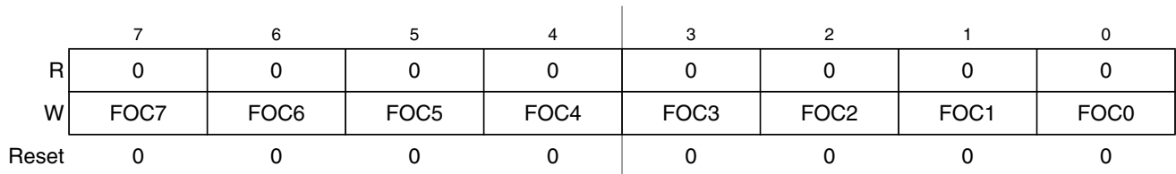
Figure 20-7. Timer Compare Force Register (CFORC)
