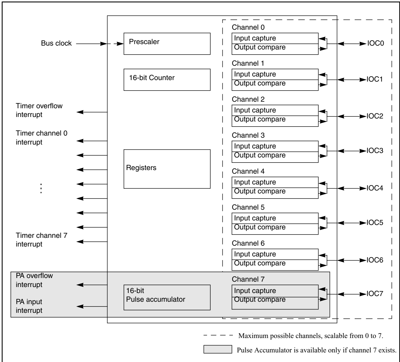
Figure 20-1. TIM16B8CV3 Block Diagram
