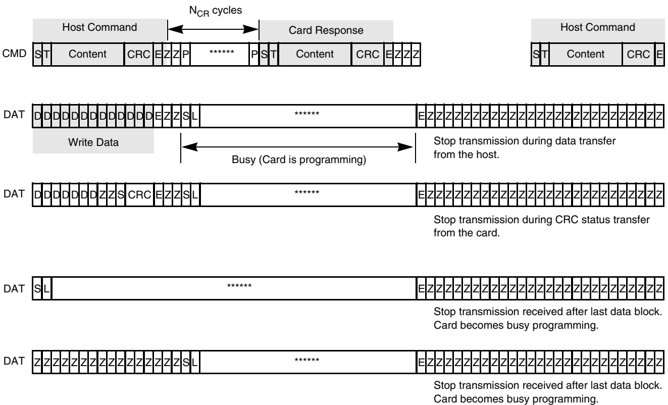
Figure 52. Stop Transmission During Different Scenarios
