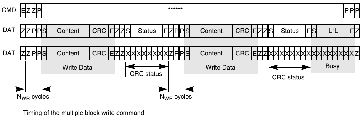
Figure 51. Timing Diagrams at Data Write
