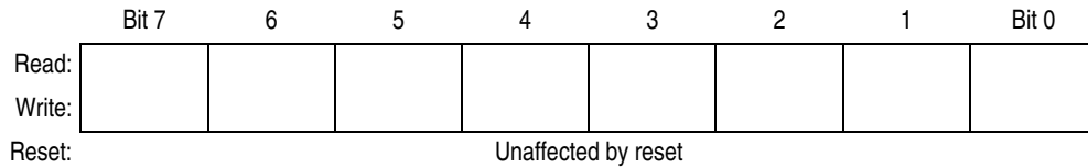
Figure 14-2. Accumulator (A)
