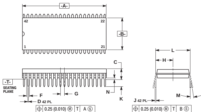
Figure 11-2 42-pin SDIP Package
