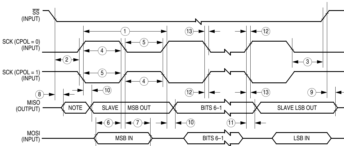
b) SPI Slave Timing (CPHA = 1)
