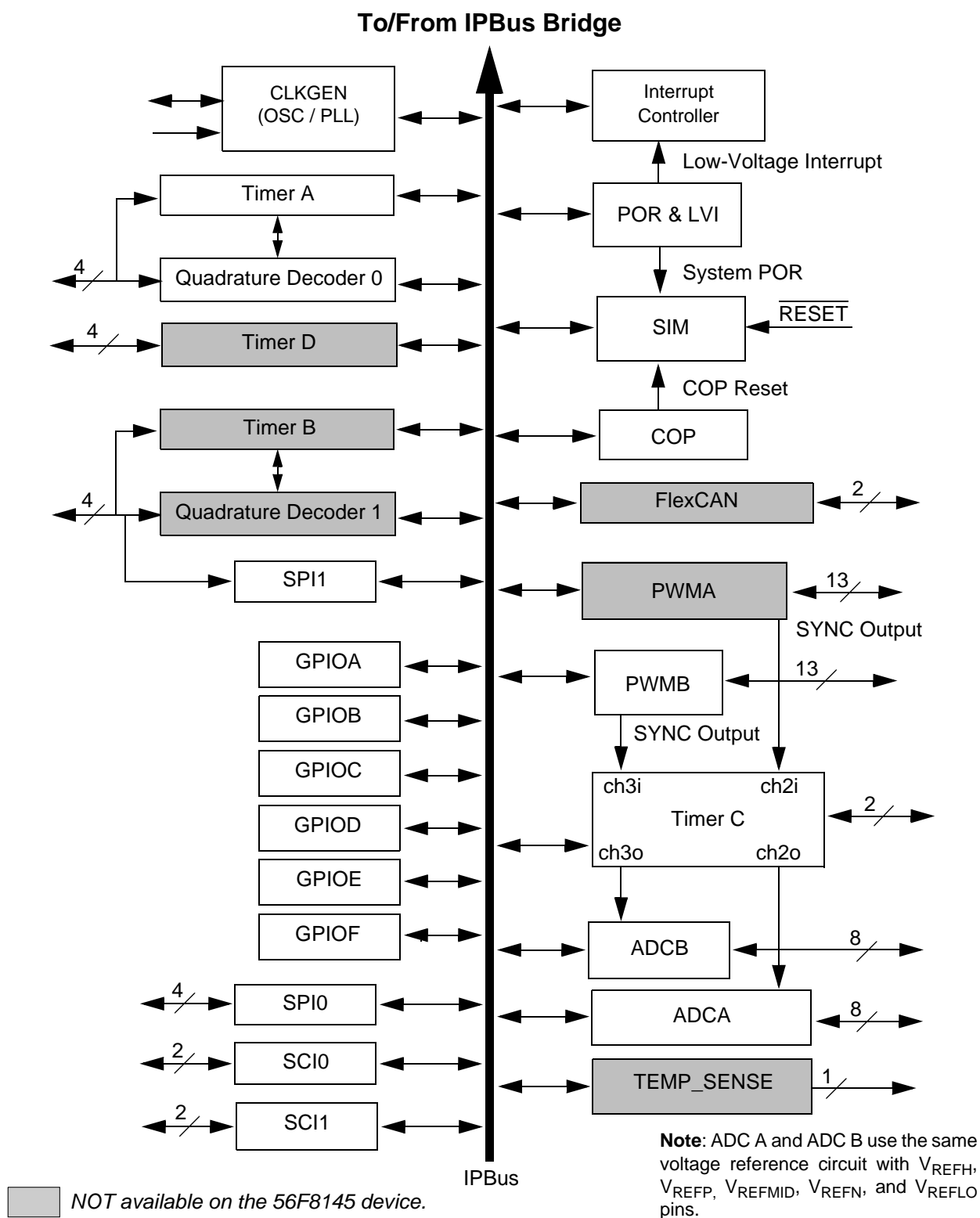
Figure 1-2 Peripheral Subsystem
