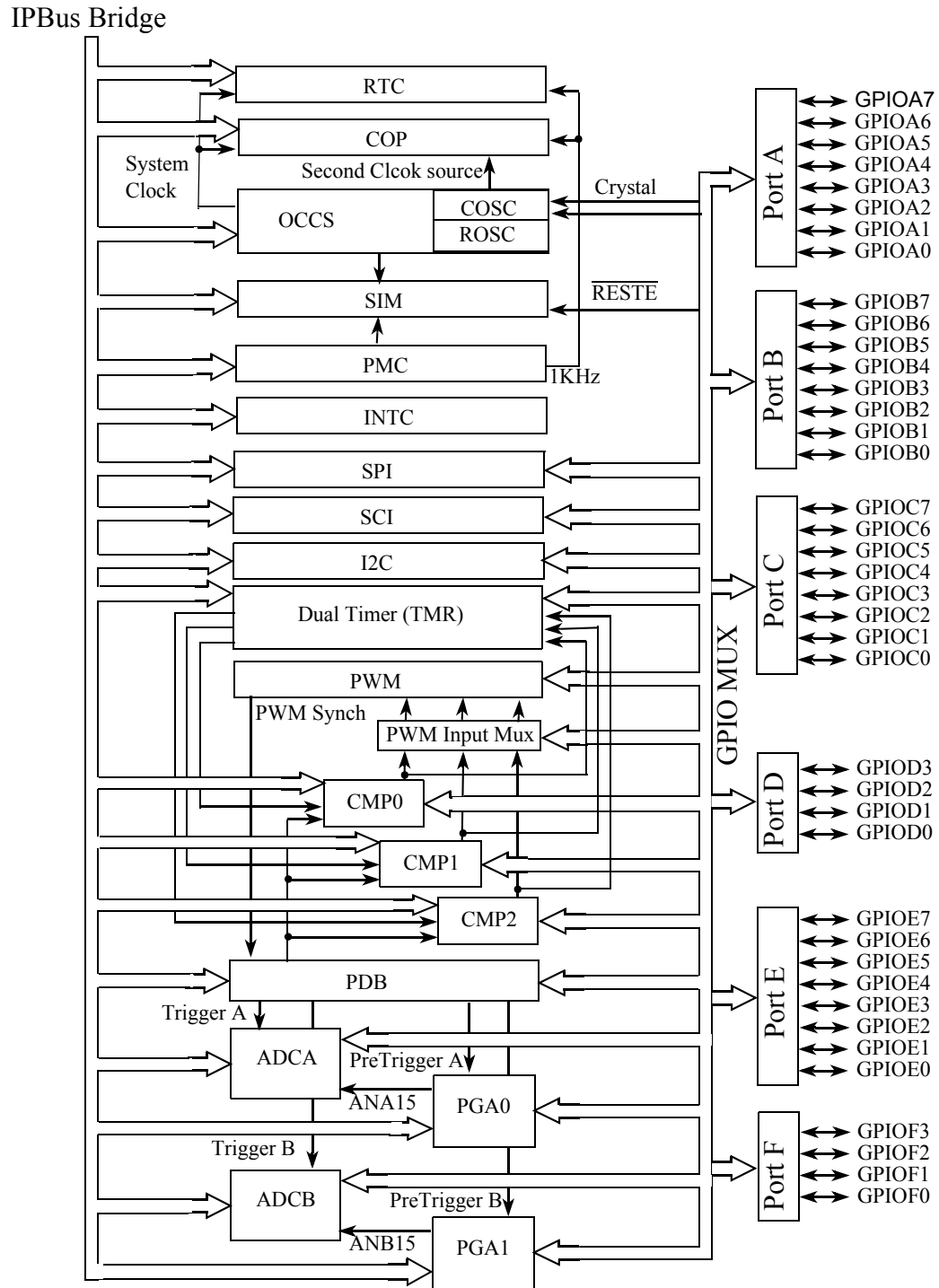
Figure 3. Peripheral Subsystem
