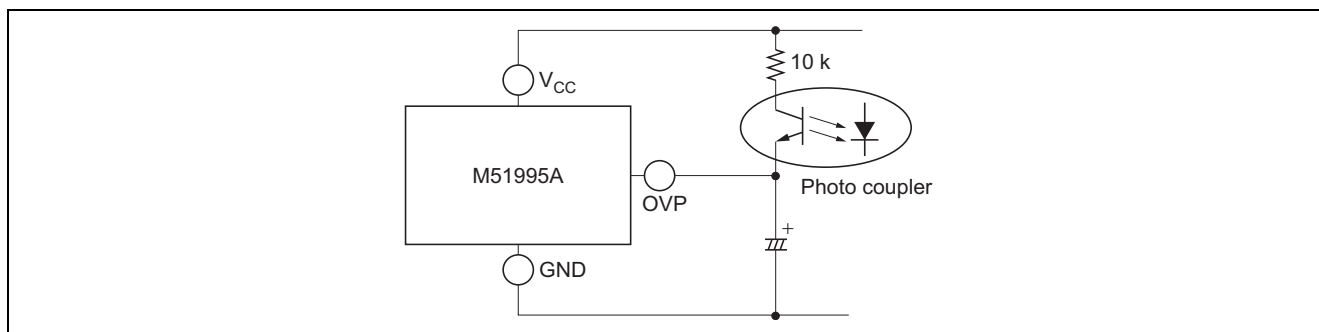
Figure 26 Peripheral Circuit of OVP Terminal
