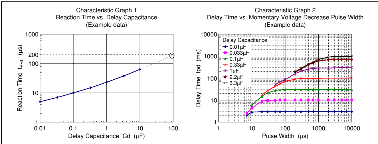
Figure 5 Characteristic Graph
