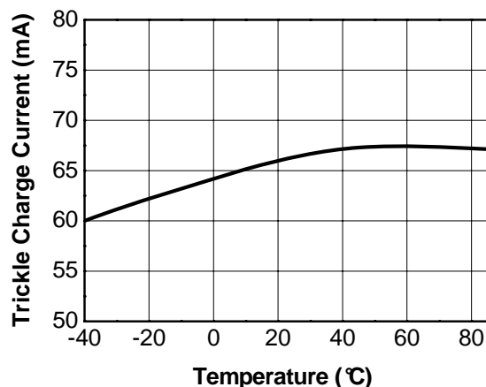
Figure 12. Trickle Charge Current vs Temperature I_{CHG} = 650\text{ mA} , V_{IN} = 5.0\text{ V} , V_{BAT} = 2\text{ V}
