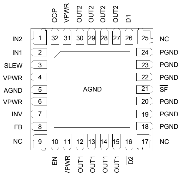
Figure 3. 33926 Pin Connections
