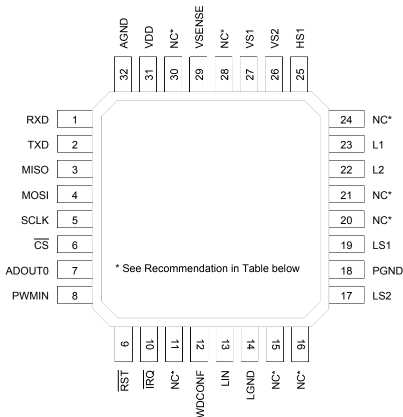
Figure 3. 33911 Pin Connections
