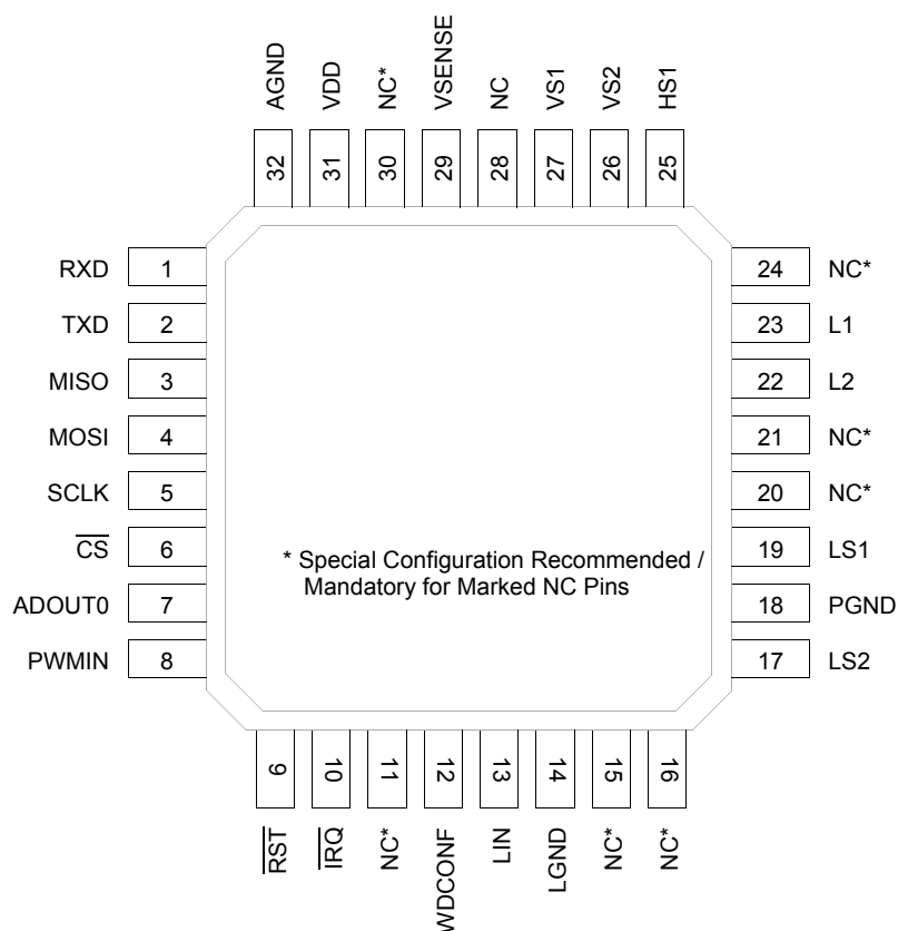
Figure 26. 33911 Pin Connections
