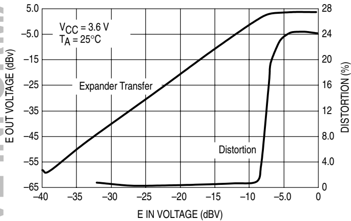
Figure 31. E In to E Out Transfer Curve
