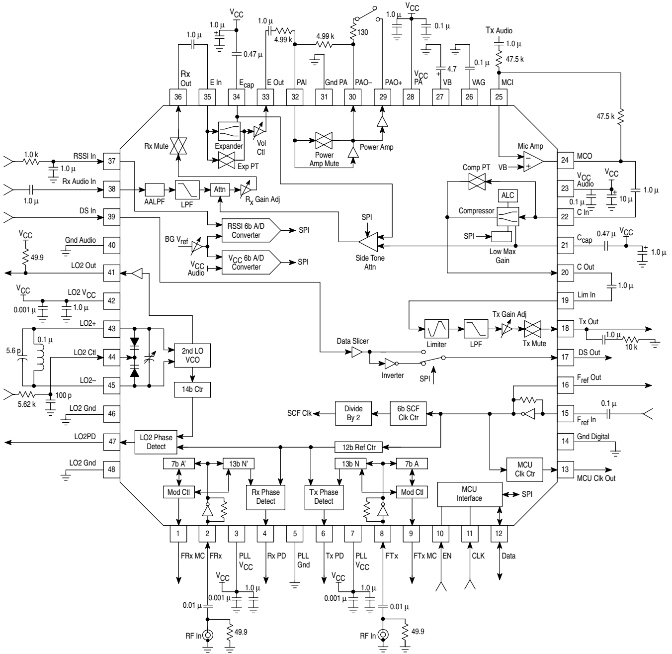
Figure 1. Test Circuit
