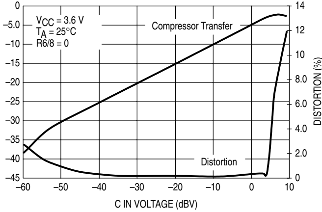
Figure 17. Tx Audio Compressor Response (Distortion & Amplitude, ALC off, Lim off)
