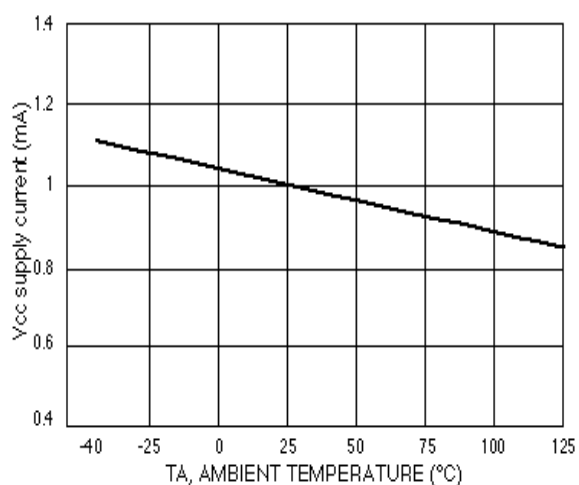
Figure 8. ICC Supply Current versus Temperature
