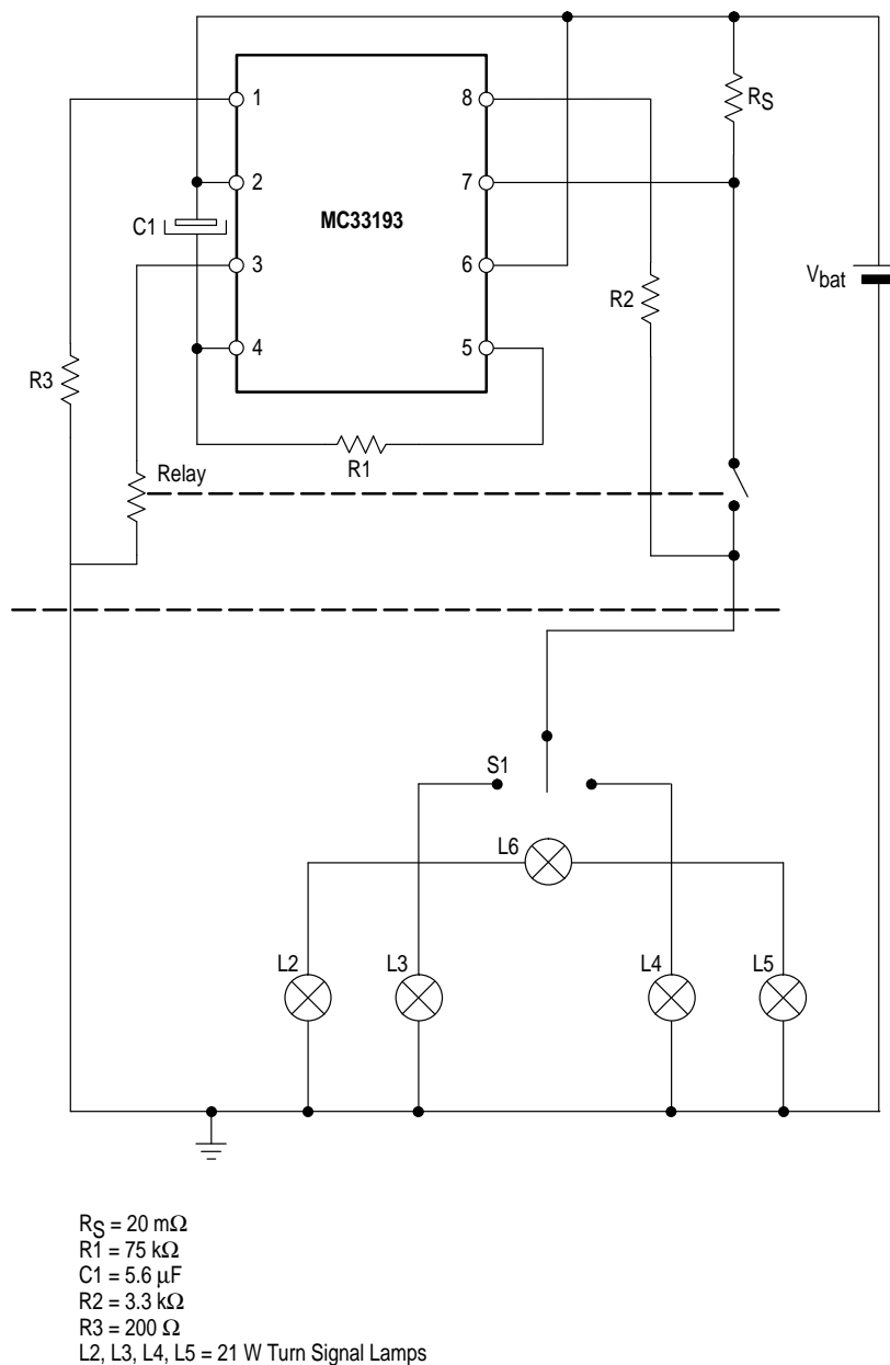
Figure 9. MC33193 Typical Application
