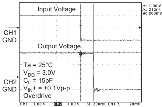
Figure 3-17 HA1631S03 TP_{HL} Transient Response (Overdrive = \pm 0.1\text{Vp-p} )
