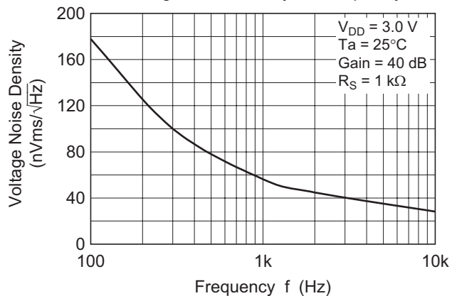
Figure 2-24. HA1630D05 Voltage Noise Density vs. Frequency
