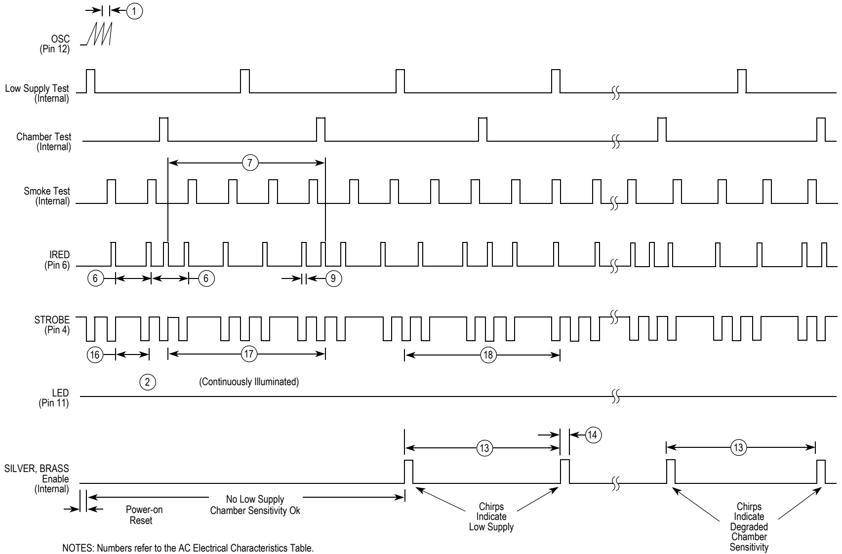
Figure 6. Standby Timing Diagram
