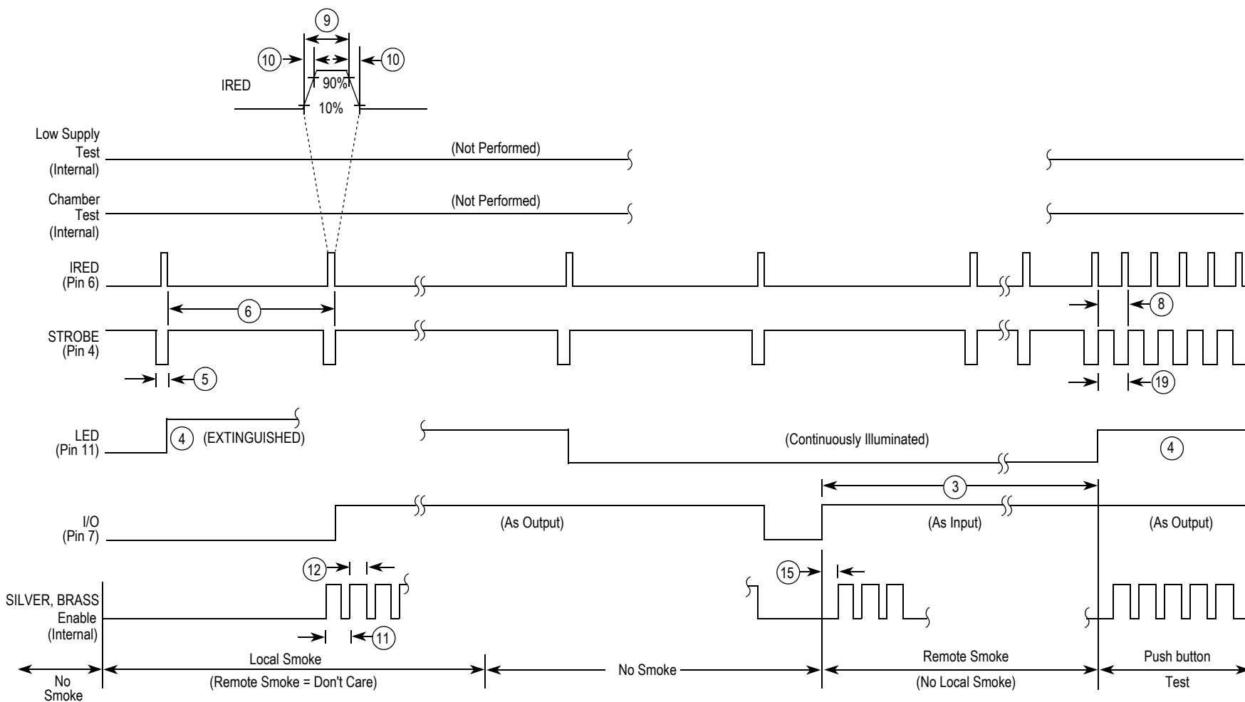
Figure 7. Smoke Timing Diagram
