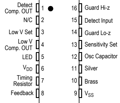
Figure 1. Pin Connections
