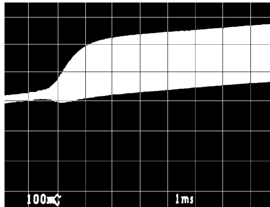
Figure 26. Oscillator Enable Time, T_{enable}
