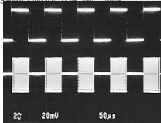
Figure 25. ASK Input Waveform and Modulated Carrier
