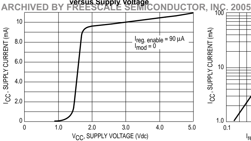
Figure 3. Supply Current versus Supply Voltage
