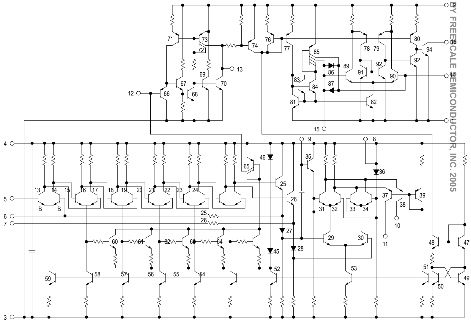
Figure 15. Internal Schematic
