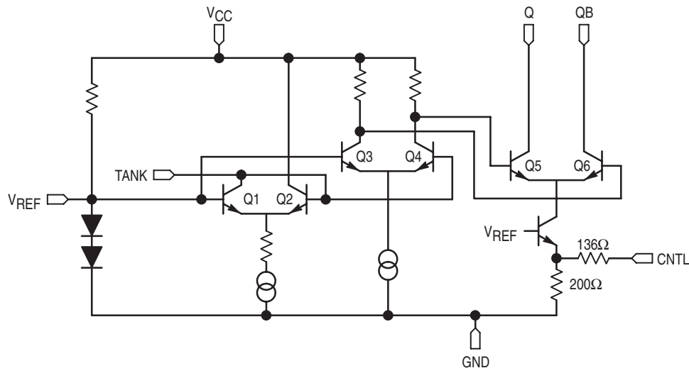
Figure 1. Simplified Schematic
