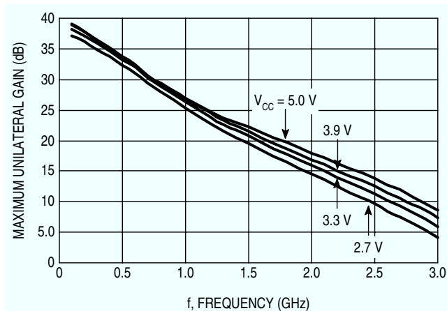
Figure 2. GUmex versus Frequency
