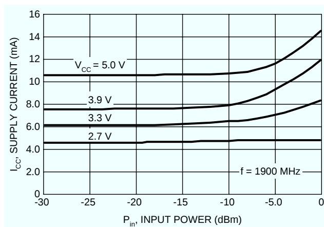
Figure 6. Supply Current versus Input Power
