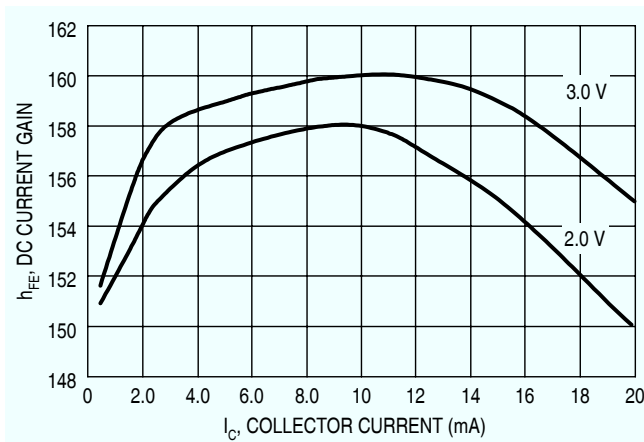
Figure 3. h_{FE} , DC Current Gain versus Collector Current
