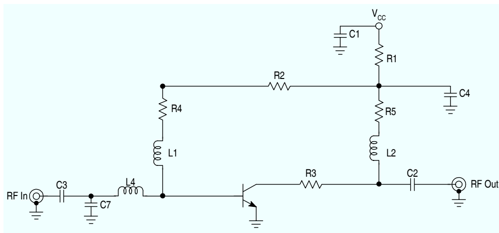
Figure 20. 1900 MHz LNA Schematic
