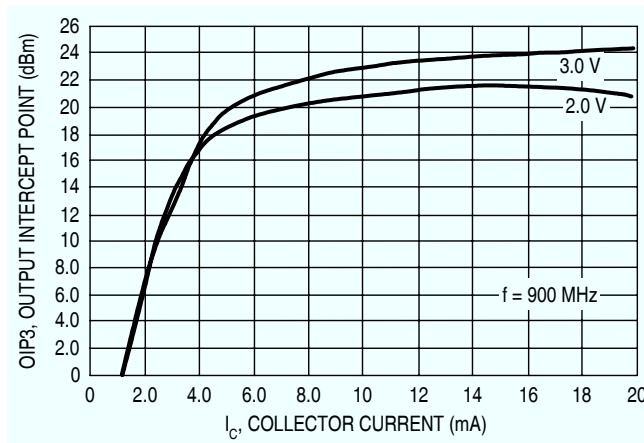
Figure 14. Output Third Order Intercept versus Collector Current
