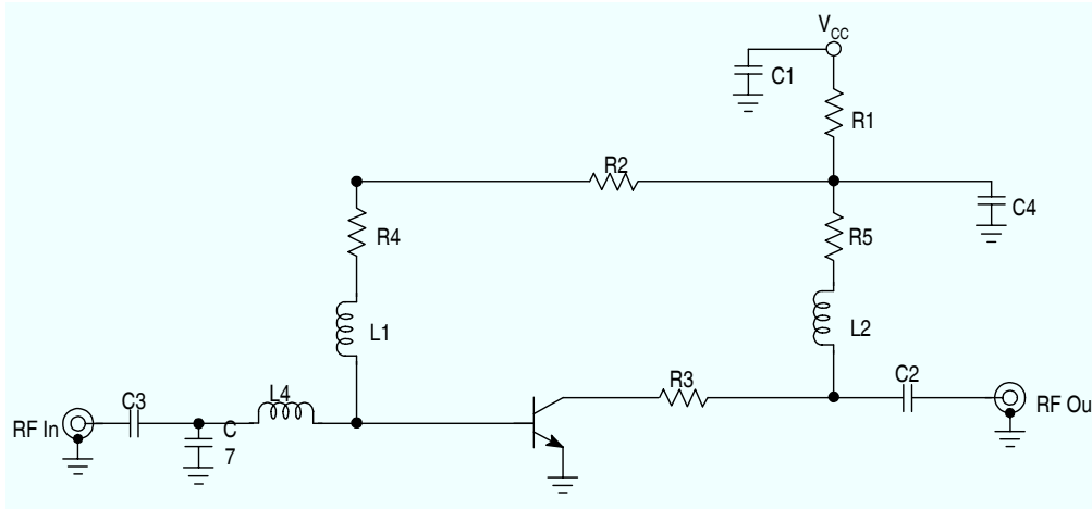
Figure 18. 900 MHz LNA Schematic
