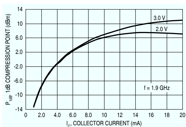
Figure 17. One dB Compression Point versus Collector Current
