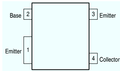
Figure 1. Pin Connections
