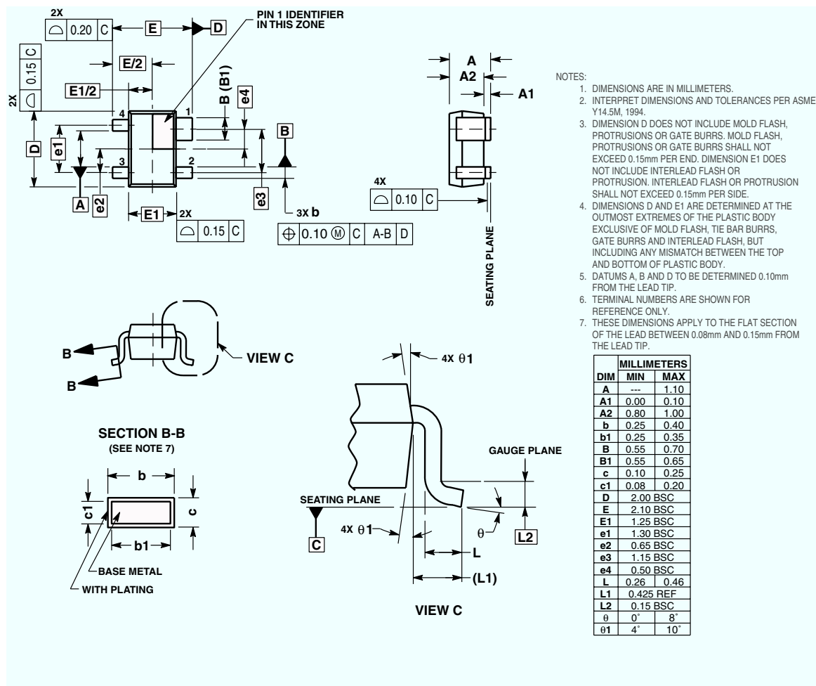
Figure 27. Outline Dimensions for SOT-343 (Case 318M-01, Issue 0)
