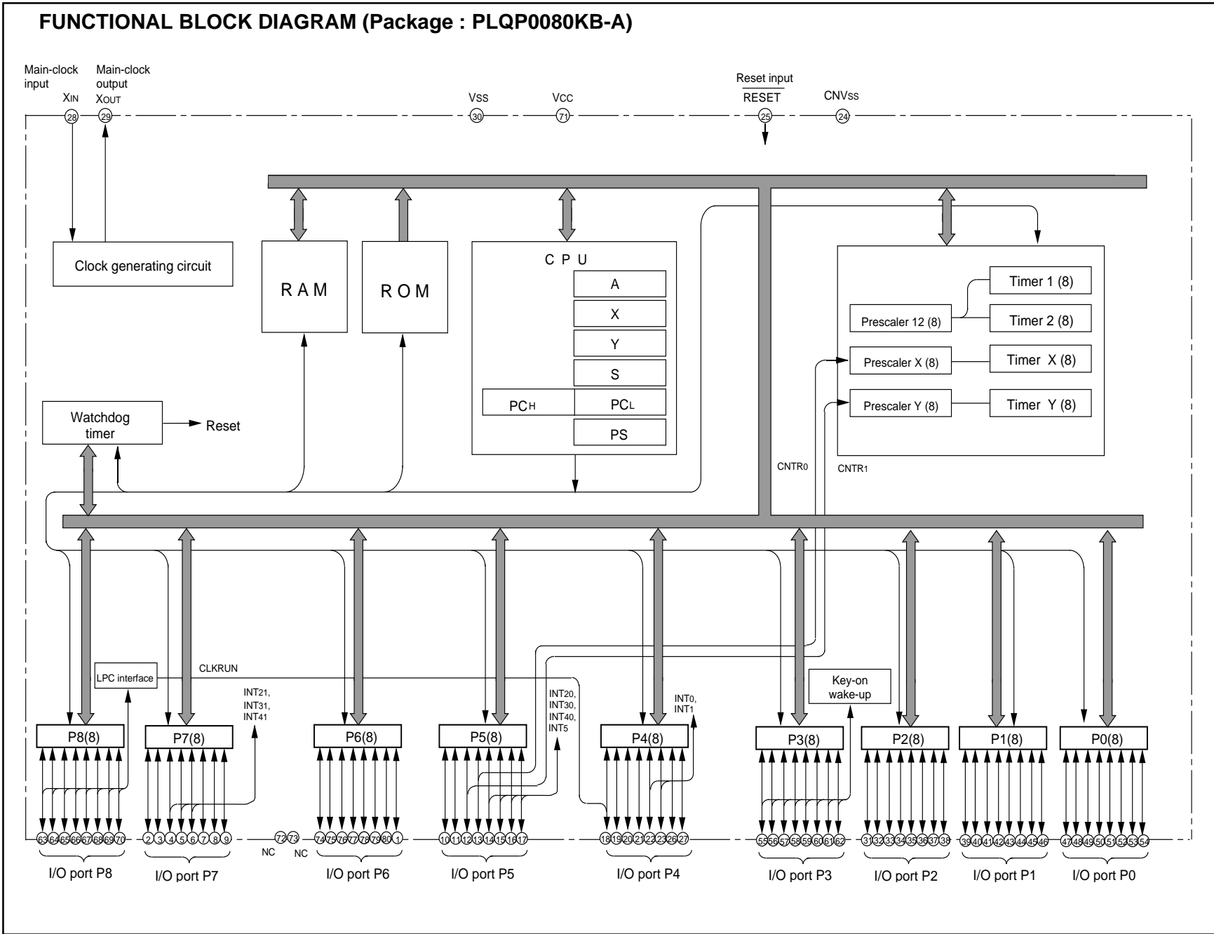
Fig. 2 Functional block diagram
