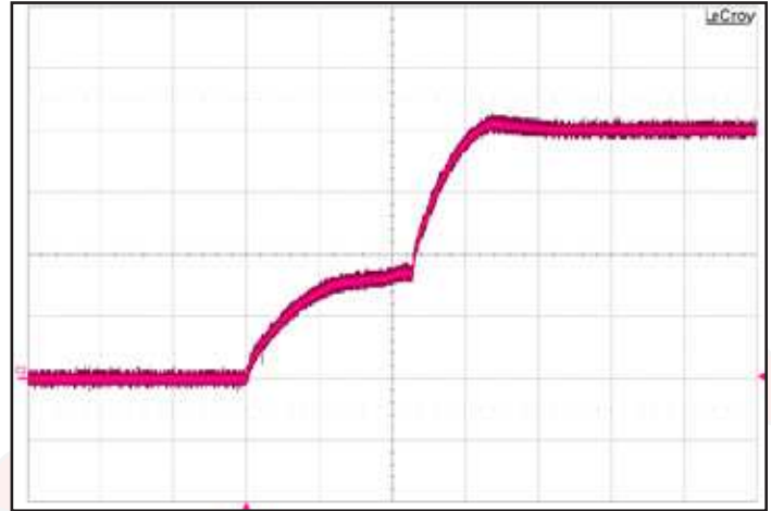
Figure 8: Output voltage startup waveform (115VAC, 60Hz) Pink: (100V/div), Timebase: (500ms/div)
