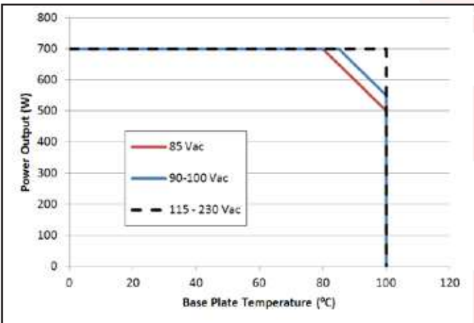
Figure 9: Derating curve for 50-60Hz input voltage.
