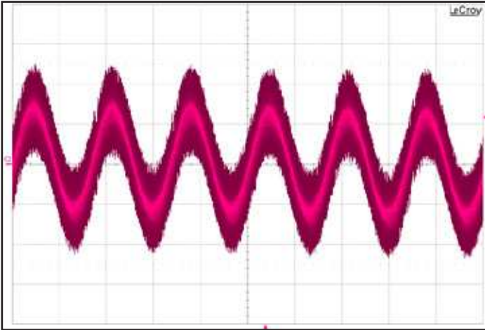
Figure 7: Output voltage with 500µF Hold-up capacitor at full rated power (115VAC, 60Hz) Pink: Vout (5V/div), Timebase: (5ms/div).
