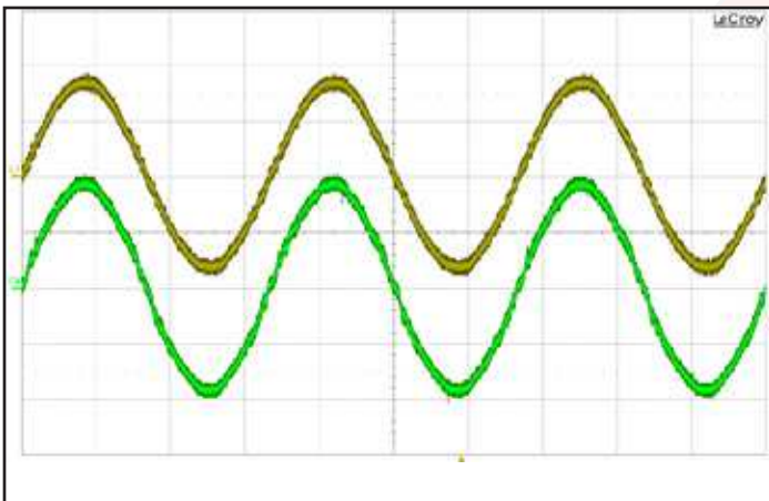
Figure 3: Typical Input Voltage and Current waveforms at full rated power (115VAC, 60Hz) Yellow: V_{in} (100V/div), Green: I_{in} (5A/div), Timebase: (5ms/div).
