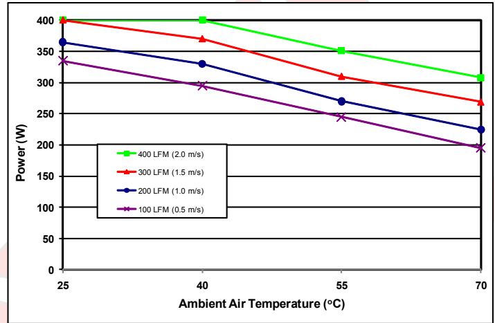
Figure 8: Power derating curves vs. ambient air temperature for airflow rates of 100 LFM through 400 LFM, with no conduction cooling.
