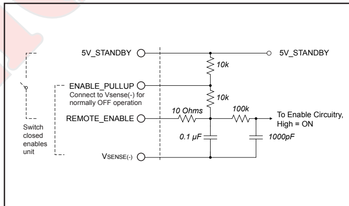
Figure C: Remote enable interface circuitry for normally OFF operation.
