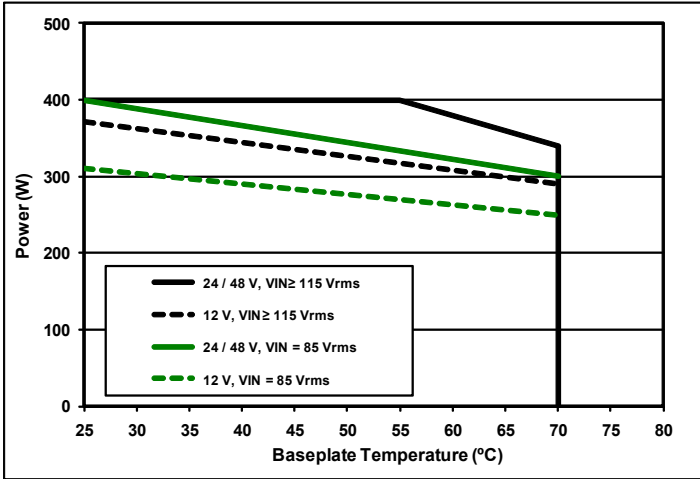
Figure 7: Continuous power derating curve for conduction cooling through flat side of chassis, with only natural convection air cooling.
