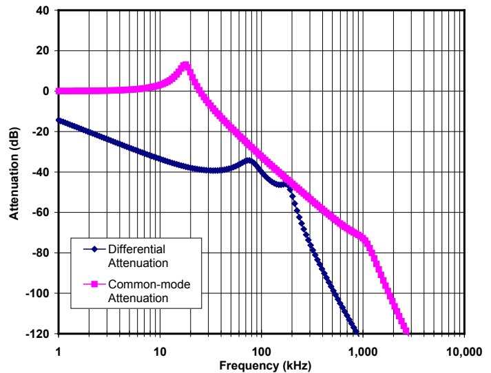
Figure 1: Typical Common Mode and Differential Mode Attenuation provided by the filter as a function of frequency. both input lines are connected to chassis ground through 50Ω resistors.
