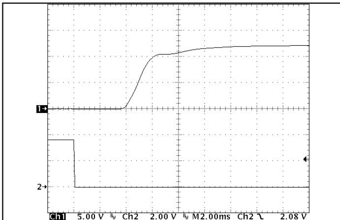
Figure 9: Turn-on transient at half load (resistive load) and 3 mF output capacitance (2.0 ms/div). Input voltage pre-applied. CH1: Vout (5V/div). CH2: ON/OFF input (2V/div). Vin = 48 V.
