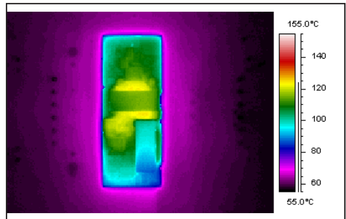
Figure 8: Thermal plot of converter at 13.5 A load current (max 125°C derating current) with 55°C air flowing at the rate of 200 LFM. Air is flowing across the converter from output to input (nominal input voltage).
