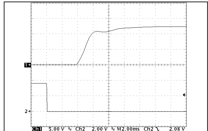
Figure 10: Turn-on transient at zero load and 3 mF output capacitance (2.0 ms/div). Input voltage pre-applied. CH1: Vout (5 V/div). CH2: ON/OFF input (2 V/div). Vin = 48 V.
