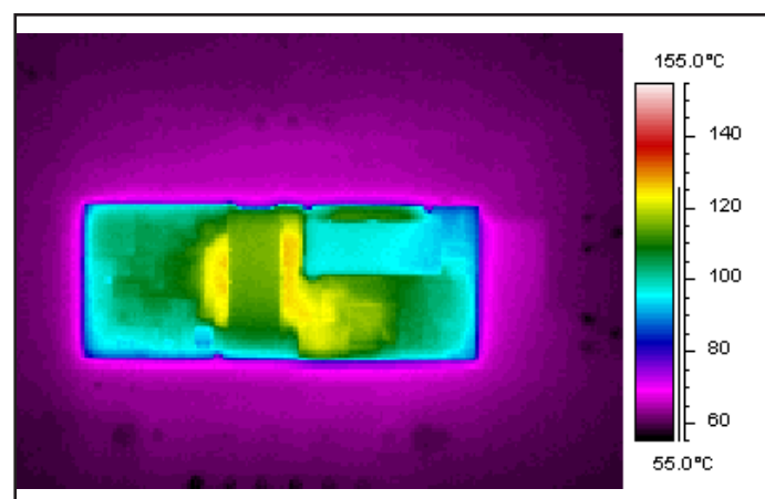
Figure 6: Thermal plot of converter at 14.7 A load current (maximum 125°C derating current) with 55°C air flowing at the rate of 200 LFM. Air is flowing across the converter from pin 3 to pin 1 (nominal input voltage).
