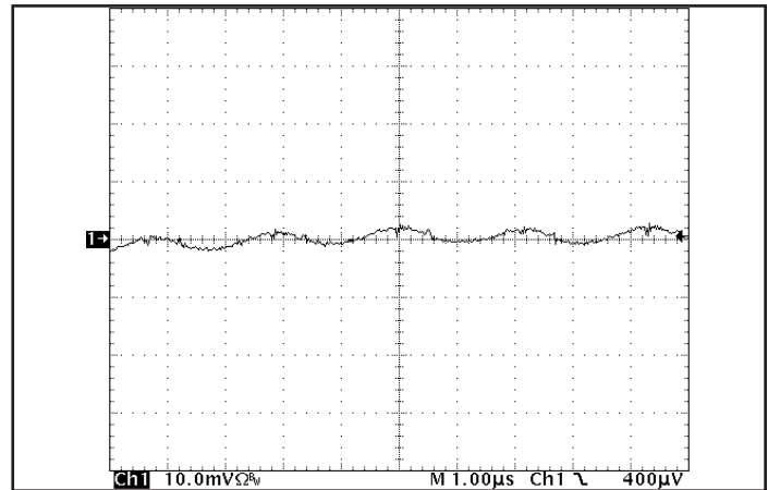
Figure 14: Input reflected ripple current, i_s , through a 10\ \mu\text{H} source inductor at nominal input voltage and rated load current (10 mA/div). See Figure 12.
