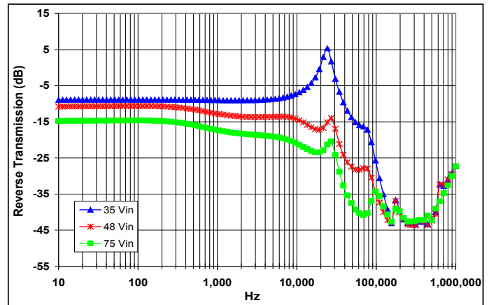
Figure 20: Magnitude of incremental reverse transmission for minimum, nominal, and maximum input voltage at full rated power.
