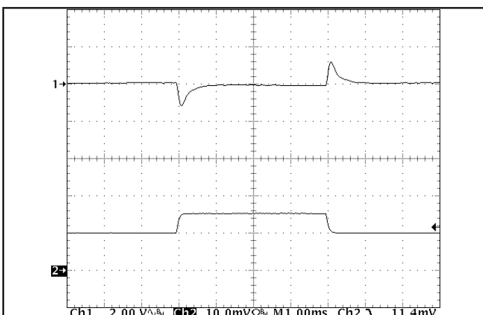
Figure 11: Output voltage response to step-change in load current (50%-75%-50%) of Iout (max); dI/dt = 0.1 A/μs. Load cap 100 μF, 100 mΩ ESR tantalum cap. Top trace: Vout (2 V/div), Ch2: Iout (10A/div). Vin = 48 V
