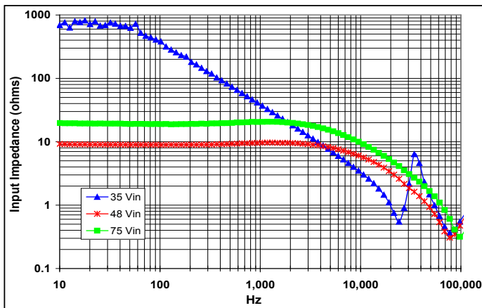
Figure 21: Magnitude of incremental input impedance for minimum, nominal, and maximum input voltage at full rated power.
