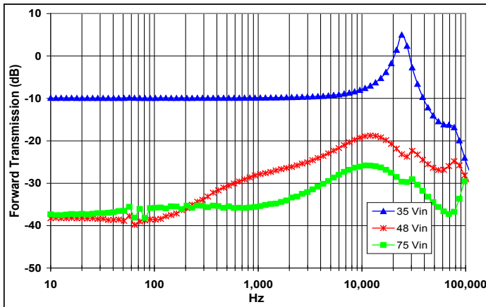
Figure 19: Magnitude of incremental forward transmission for minimum, nominal, and maximum input voltage at full rated power.
