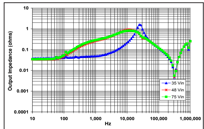
Figure 18: Magnitude of incremental output impedance for minimum, nominal, and maximum input voltage at full rated power.
