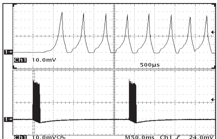
Figure 17: Load current (10 A/div) as a function of time when the converter attempts to turn on into a 1m\Omega short circuit. Top trace (500 us/div) is an expansion of the on-time portion of the bottom trace.
