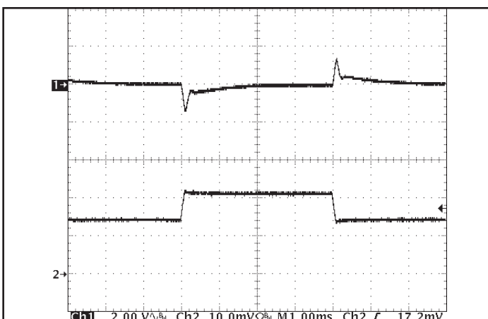
Figure 11: Output voltage response to step-change in load current (50%-75%-50% of Iout(max); dI/dt = 0.1A/\mu s ). Load cap: 100 \mu F, 100 m \Omega ESR tantalum cap and 1 \mu F ceramic cap. Ch 1: Vout (2 V/div), Ch 2: Iout (10A/div).
