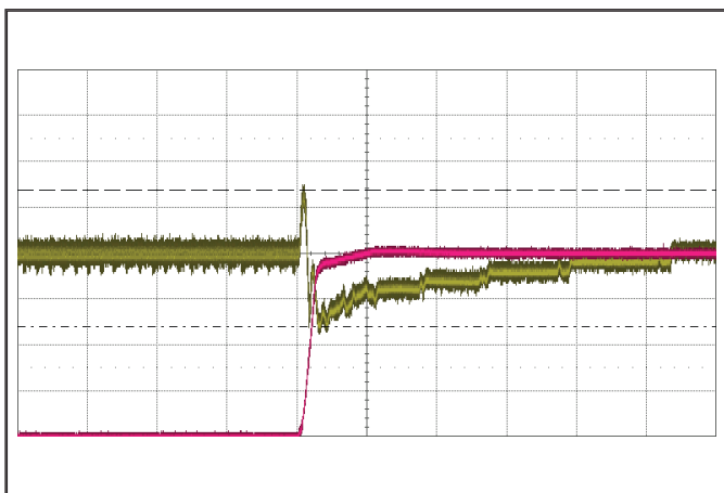
Figure 15: Output voltage response to step-change in input voltage (35 V to 75V in 300 \mu\text{s} ; 1 ms/div). Load cap: 470 \mu\text{F} , 15 mW ESR electrolytic capacitor. Top trace: V_{\text{out}} (500 mV/div). Bottom trace: V_{\text{in}} (10 V/div), at zero load current.
