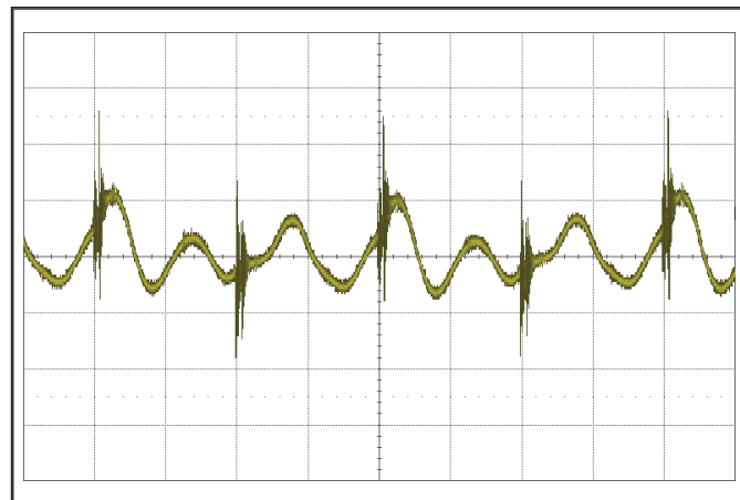
Figure 14: Output voltage ripple at nominal input voltage and rated load current (50 mV/div; 2 \mu\text{s} /div). Load capacitance: 1 \mu\text{F} ceramic capacitor and 15 \mu\text{F} tantalum capacitor. Bandwidth: 20 MHz. See Figure 11.
