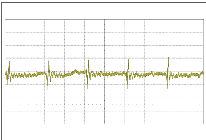
Figure 13: Input reflected ripple current, is, through a 4.7 \mu\text{H} source inductor, using a 220 \mu\text{F} input capacitor, at nominal input voltage and rated load current (10 mA/div; 2 \mu\text{s} /div). See Figure 11.
