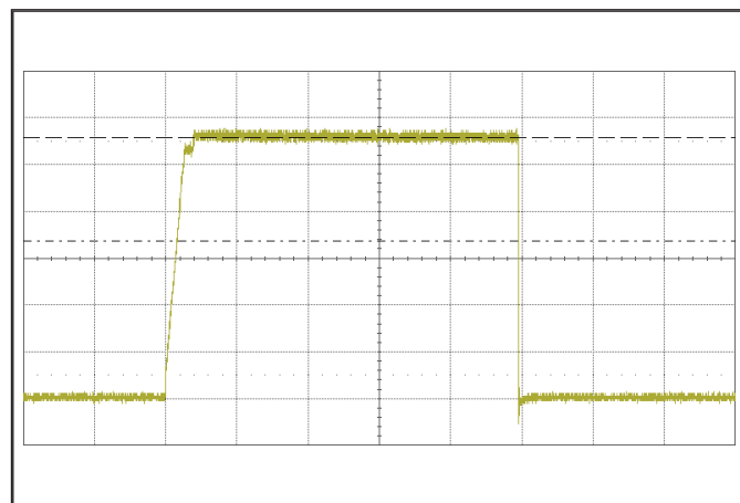
Figure 16: Load current (10 A/div; 10 ms/div) as a function of time when the converter attempts to turn on into a 1 mW short circuit.
