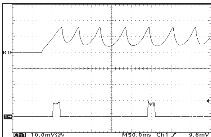
Figure 18: Load Current (50A/div) as a function of time when the converter attempts to turn on into a 1 mΩ short circuit. Top trace (500µs/div) is an expansion of the on-time portion of the bottom trace. V_{in} = 48V
