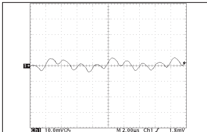
Figure 15: Input reflected ripple current, i_s , through a 10µH source inductor; using a 47µF electrolytic input capacitor (20mA/div) at nominal input voltage and rated load current. See Figure 13.
