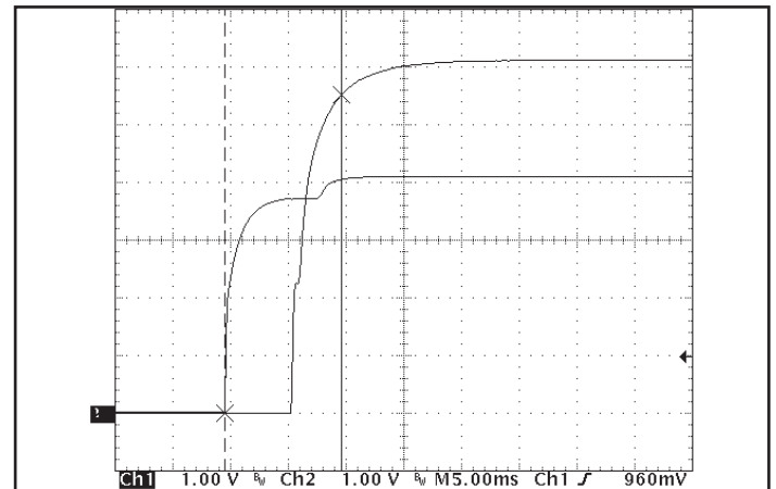
Figure 10: Turn-on transient at zero load (5.0ms/div). Load cap: 15µF, 100mΩ ESR tantalum capacitor and 1µF ceramic capacitor. Input voltage pre-applied. CH1: V_{out} (1V/div). CH2: ON/OFF input (1V/div). V_{in} = 48V.
