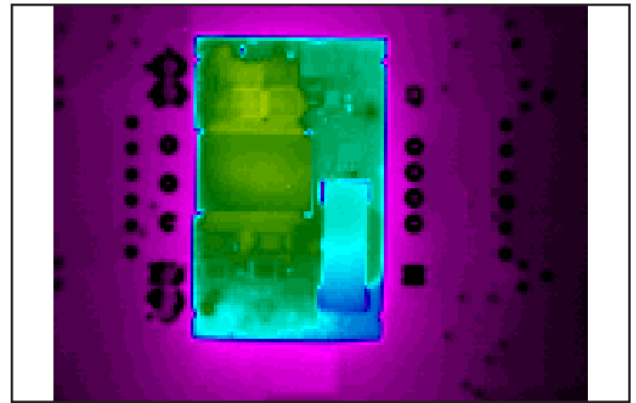
Figure 8: Thermal plot of converter at 43A load current (252 W) with 55°C air flowing at the rate of 200 LFM. Air is flowing across the converter from output to input (nominal input voltage).
