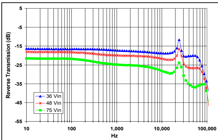
Figure 21: Magnitude of incremental reverse transmission for minimum, nominal, and maximum input voltage at full rated power.
