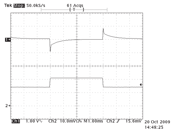
Figure 12: Output voltage response to step-change in load current (50%-75%-50%) of I_{out} (max); dI/dt = 1A/µs. Load cap 15µF, 100mΩ ESR tantalum capacitor and 1µF ceramic capacitor. Ch 1: V_{out} (1V/div), Ch 2: I_{out} (20A/div). V_{in} = 48V
