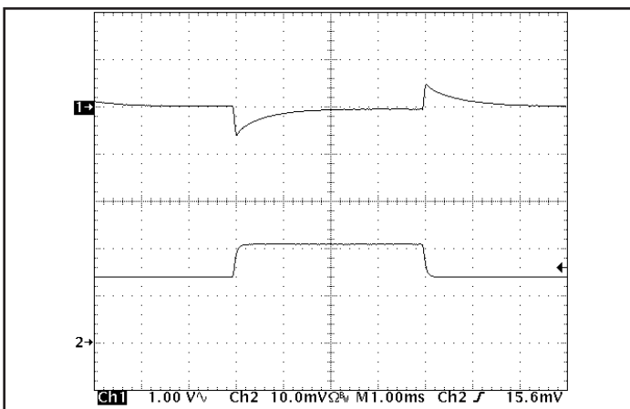
Figure 11: Output voltage response to step-change in load current (50%-75%-50%) of I_{out} (max); dI/dt = 0.1A/µs. Load cap 15µF, 100mΩ ESR tantalum capacitor and 1µF ceramic capacitor. Ch 1: V_{out} (1V/div), Ch 2: I_{out} (20A/div). V_{in} = 48V
