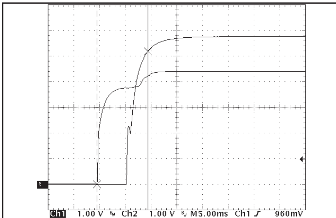
Figure 9: Turn-on transient at full load (resistive load) (5.0ms/div). Load cap: 15µF, 100mΩ ESR tantalum capacitor and 1µF ceramic capacitor. Input voltage pre-applied. CH1: V_{out} (1V/div). CH2: ON/OFF input (1V/div). V_{in} = 48V.
