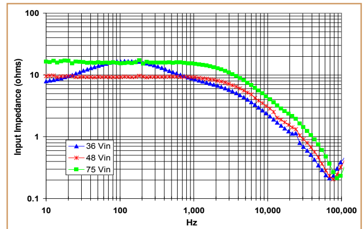
Figure 22: Magnitude of incremental input impedance for minimum, nominal, and maximum input voltage at full rated power.
