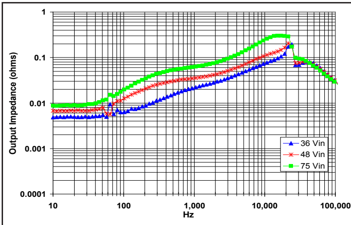
Figure 19: Magnitude of incremental output impedance for minimum, nominal, and maximum input voltage at full rated power.
