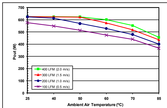
Figure 6: Maximum output power derating curve vs. ambient air temperature (with both baseplate and heat sink) at different airflow rates with air flowing from output to input (nominal input voltage).
