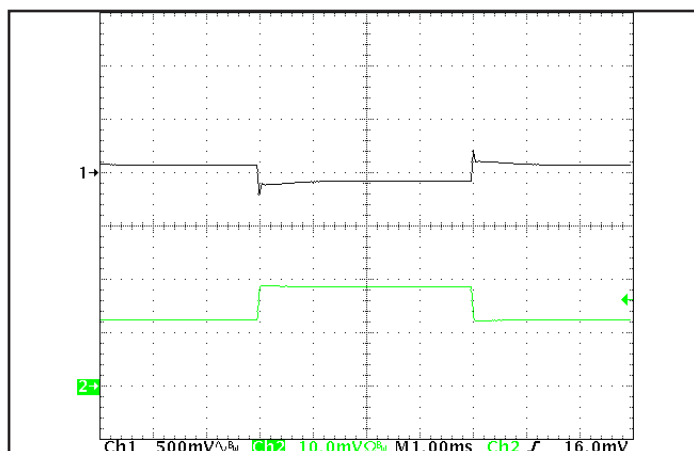
Figure 12: Output voltage response to step-change in load current (50%-75%-50% of Iout(max); dI/dt = 1A/μs). Load cap: 15μF, 30mΩ ESR tantalum cap and 1μF ceramic cap. Ch 1: Vout (500mV/div), Ch 2: Iout (20A/div).
