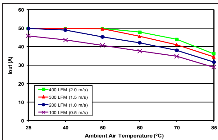
Figure 5: Maximum output current derating curve vs. ambient air temperature (with both baseplate and heat sink) at different airflow rates with air flowing from output to input (nominal input voltage).
