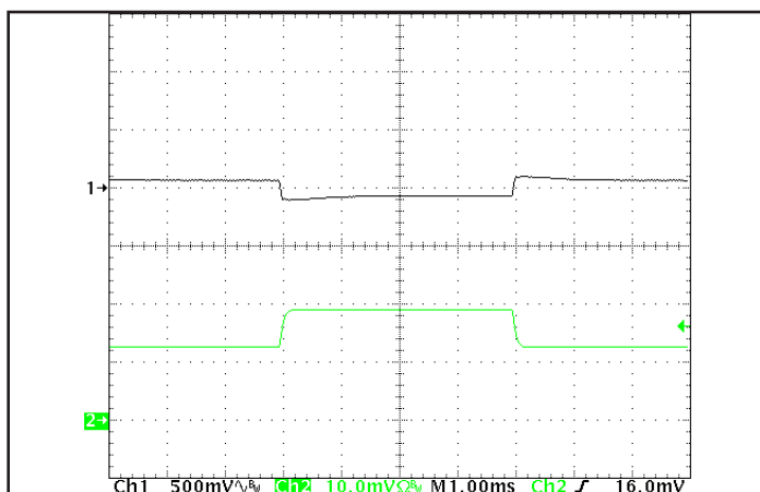
Figure 11: Output voltage response to step-change in load current (50%-75%-50% of Iout(max); dI/dt = 0.1A/μs). Load cap: 15μF, 30mΩ ESR tantalum cap and 1μF ceramic cap. Ch 1: Vout (500mV/div), Ch 2: Iout (20A/div).
