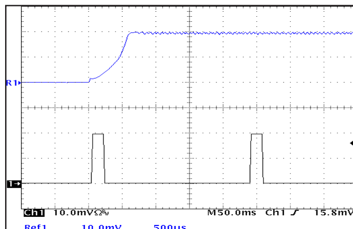
Figure 18: Load current (50A/div) as a function of time when the converter attempts to turn on into a 1mΩ short circuit. Top trace (500µs/div) is an expansion of the on-time portion of the bottom trace.
