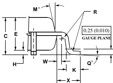
Figure 4-2 100-pin LQFP Mechanical Information
