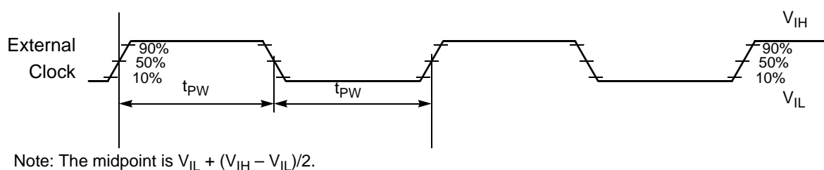
Figure 3-10 External Clock Timing
