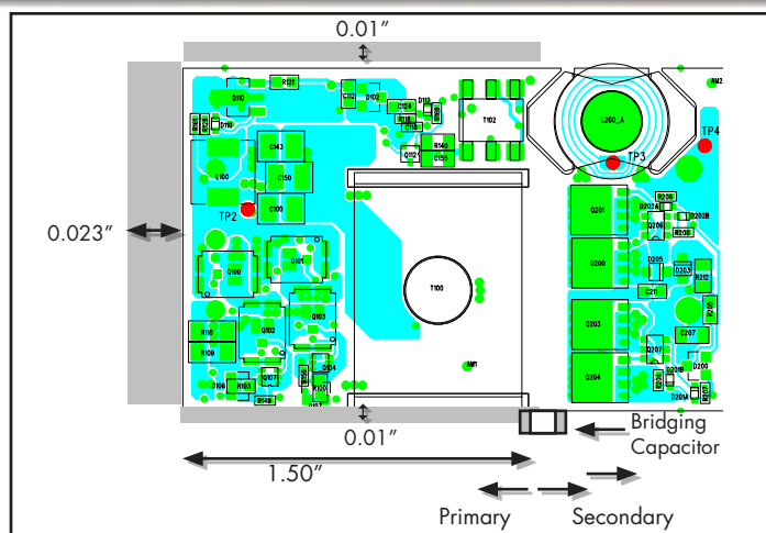
Figure F: Keep Out Areas for BusQor module
