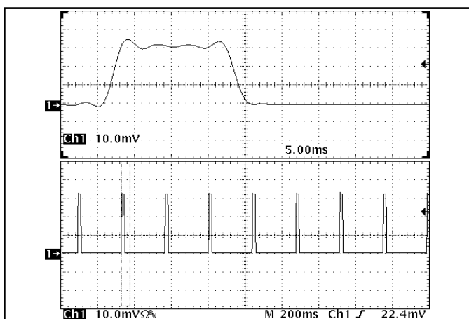
Figure 17: Load current (10A/div) as a function of time when the converter attempts to turn on into a 1 mΩ short circuit. Top trace (5.0ms/div) is an expansion of the on-time portion of the bottom trace.
