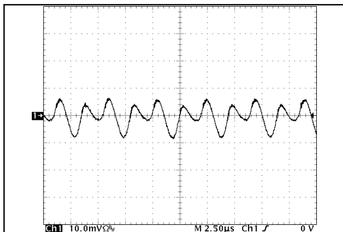
Figure 13: Input Terminal Ripple Current, i_C , at full rated output current and nominal input voltage with 10 H source impedance and 47 F electrolytic capacitor (50 mA/div). See Figure 12.
