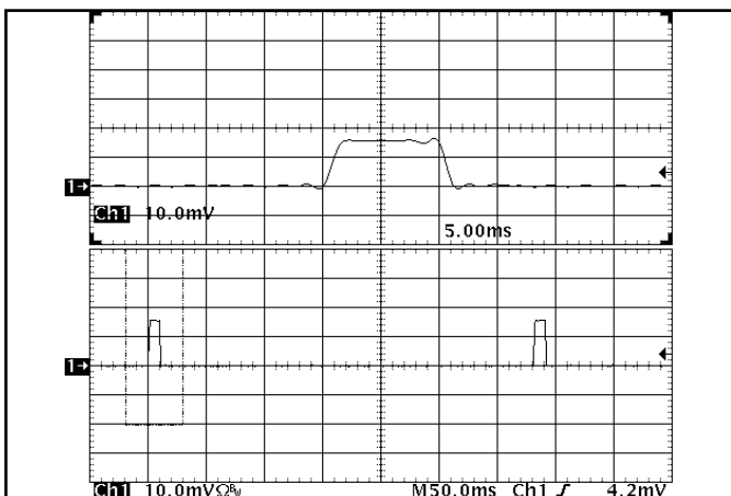
Figure 17: Load current (50A/div) as a function of time when the converter attempts to turn on into a 1 m \Omega short circuit. Top trace (5.0ms/div) is an expansion of the on-time portion of the bottom trace.
