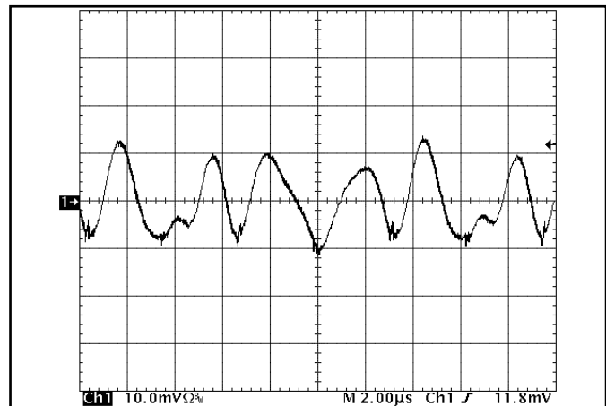
Figure 14: Input reflected ripple current, i_S , through a 10 H source inductor at nominal input voltage and rated load current (20mA/div). See Figure 12.
