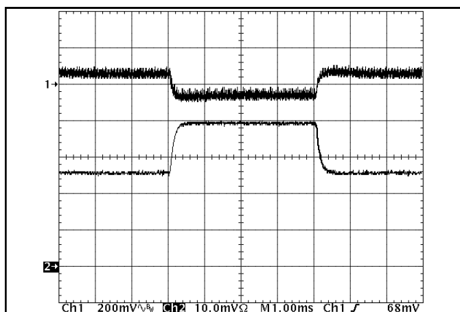
Figure 11: Output voltage response to step-change in load current (50%-75%-50% of I_{out(max)} ; dI/dt = 0.1A/s ). Load cap: 15 F, 100 mΩ ESR tantalum cap and 1 F ceramic cap. Top trace: V_{out} (200mV/div), Bottom trace: I_{out} (5A/div).
