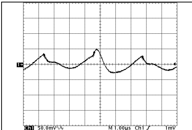
Figure 15: Output voltage ripple at nominal input voltage and rated load current (50 mV/div). Load capacitance: 1 F ceramic capacitor and 15 F tantalum capacitor. Bandwidth: 20 MHz. See Figure 12.
