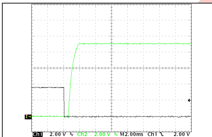
Figure 9: Turn-on transient at full load (resistive load) (2 ms/div). Load cap: 15µF tantalum capacitor and 3mF ceramic capacitor bank. Input voltage pre-applied. Ch 1: ON/OFF input (2 V/div). Ch 2: V_{out} (2V/div).
