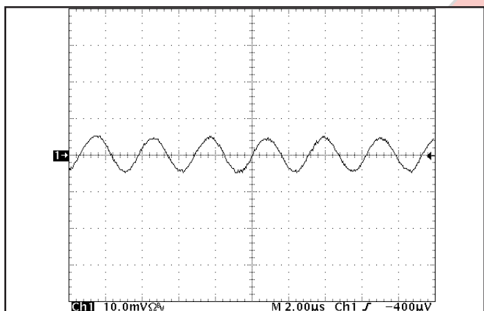
Figure 15: Input reflected ripple current, i_s , through a 10µH source inductor, using a 47µF electrolytic input capacitor (10mA/div). See Figure 13.
