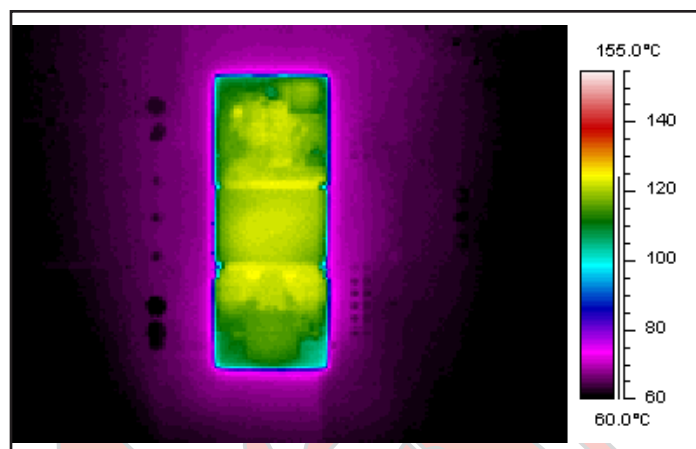
Figure 8: Thermal plot of converter 29.2 A load current (264.3 W) with 55°C air flowing at the rate of 200 LFM. Air is flowing across the converter from output to input (nominal input voltage).
