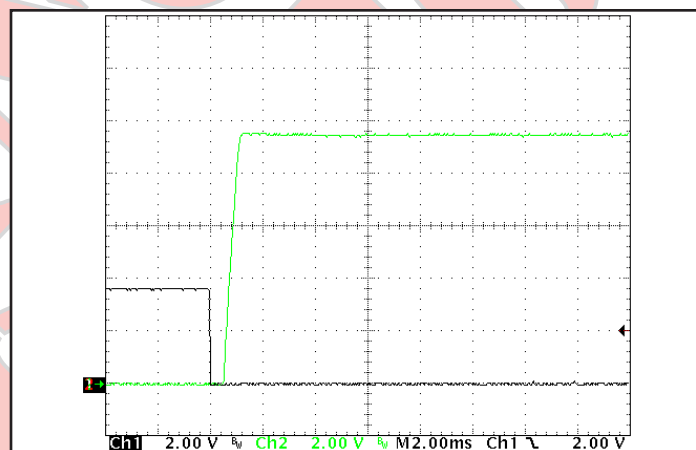
Figure 10: Turn-on transient at zero load (2 ms/div). Load cap: 15µF tantalum capacitor and 3mF ceramic capacitor bank. Ch 1: ON/OFF input (2 V/div), Ch 2: V_{out} (2V/div).
