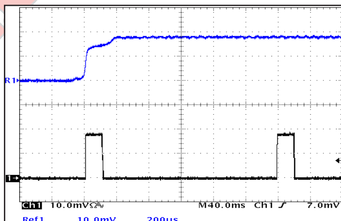
Figure 18: Load current (50A/div) as a function of time when the converter attempts to turn on into a 1mΩ short circuit. Top trace (200µs/div) is an expansion of the on-time portion of the bottom trace.
