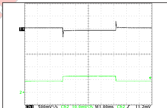
Figure 12: Output voltage response to step-change in load current (50%-75%-50% of I_{out(max)} ; dI/dt = 1A/\mu s ). Load cap: 15µF, 30 mΩ ESR tantalum cap and 1µF ceramic cap. Ch 1: V_{out} (500mV/div), Ch 2: I_{out} (20A/div).
