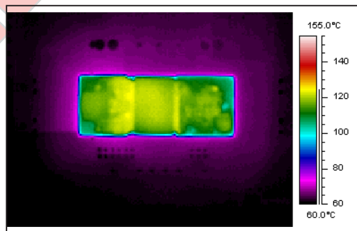
Figure 6: Thermal plot of converter at 30.9A load current (279.3W) with 55°C air flowing at the rate of 200 LFM. Air is flowing across the converter from pin 1 to pin 3 (nominal input voltage).
