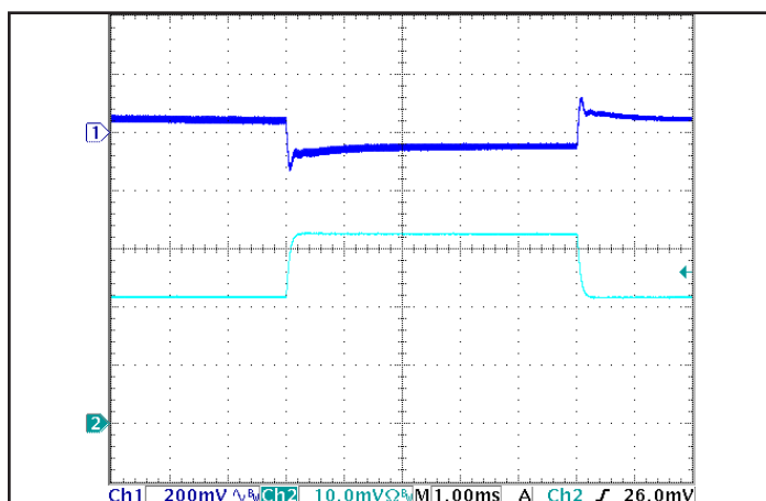
Figure 11: Output voltage response to step-change in load current (50%-75%-50% of I_{out(max)} ; dI/dt = 0.1A/\mu s ). Load cap: 15 \mu F , 100 mW ESR tantalum cap and 1 \mu F ceramic cap. Top trace: V_{out} (200mV/div), Bottom trace: I_{out} (10A/div).
