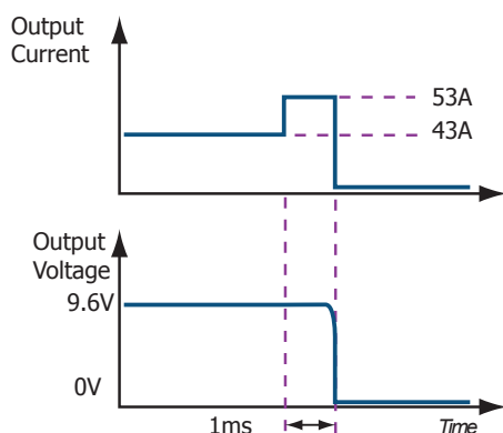
Figure C: Output Overload protection diagram (not to scale)
