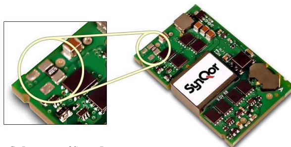
Figure G: Location of Sense Resistor
