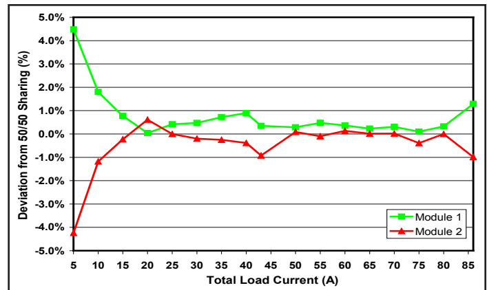
Figure I: Current share performance of 2 paralleled modules
