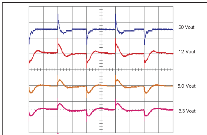
Figure 11: Output voltage response for 3.3 V, 5 V, 12 V, 20 V units to step-change in load current (50-75-50% of Iout max; di/dt=0.1A/µs). Load cap: 100µF, 100mΩ ESR tant, Ch 1-4: Vout (1 V/div);(5ms/div).
