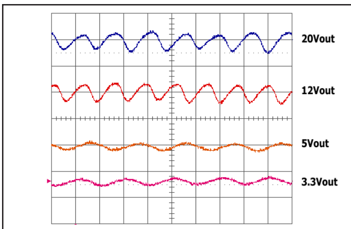
Figure 5: Input Terminal Ripple Current at 10 V input voltage and rated load current (500 mA/div). Bandwidth: 20 MHz. (See Figure 4)
