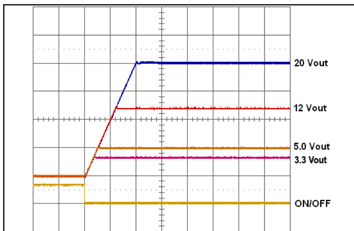
Figure 7: Turn-on transient at zero load (50 ms/div). ON/OFF input (5 V/div) Ch 1-4: Vout (5 V/div)
