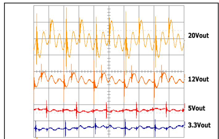
Figure 6: Output Voltage Ripple at 10 V input voltage and rated load current (20mV/div). Zero load capacitance. Bandwidth: 20 MHz. (See Figure 4)
