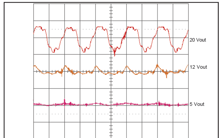
Figure 6: Output Voltage Ripple at 12V input voltage and rated load current (20mV/div). Load capacitance: 100 \mu F electrolytic cap. Bandwidth: 20MHz. (See Figure 4)
