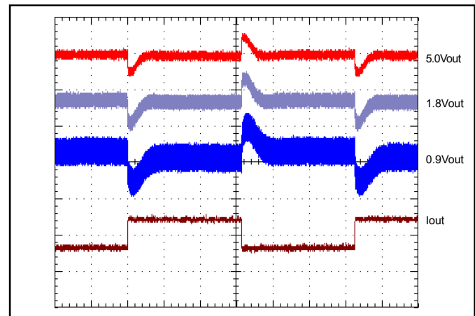
Figure 12: Output voltage response for 0.9V, 1.8V, 5V units to step-change in load current (50-75-50% of Iout max; di/dt=3A/s). Load cap: 470 F, 100mΩ ESR tant, 10 F cer. Ch 1: Iout (10A/div), Ch 2-4: Vout (100mV/div).
