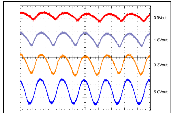
Figure 16: Output Voltage Ripple at nominal input voltage and rated load current (50 mV/div). Load capacitance: 22 F ceramic cap. Bandwidth: 20 MHz. See Figure 13.
