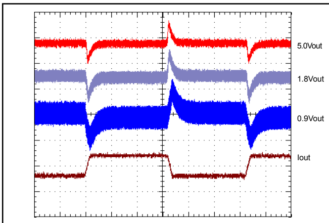
Figure 11: Output voltage response for 0.9V, 1.8V, 5V units to step-change in load current (50-75-50% of Iout max; di/dt=0.1A/s). Load cap: 100 F, 100mΩ ESR tant, 10 F cer. Ch 1: Iout (10A/div), Ch 2-4: Vout (100mV/div).
